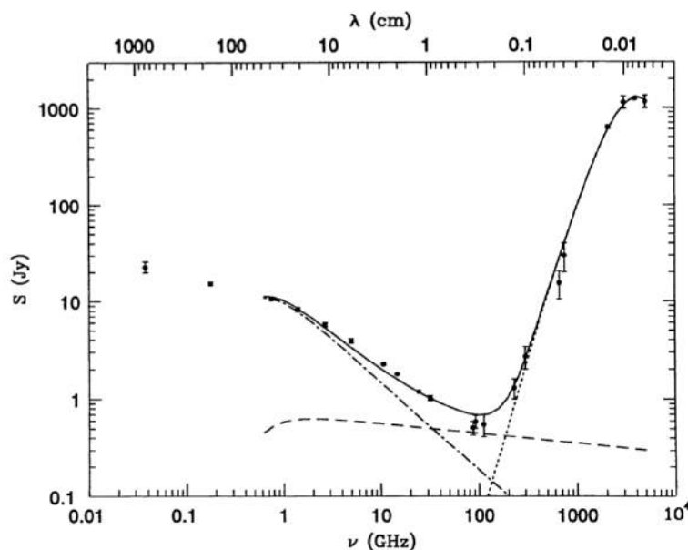
Figure 1.5: Radio/FIR Spectral Energy Distribution of M82 - The radio continuum of this starburst galaxy is the sum of three components: the steep , from \sim 1 to 30 GHz and dominated by synchrotron radiation (dot-dash line), the flat , between 30 and 100 GHz, due to thermal free-free emission (dashed line) and the inverted , dominated by thermal dust re-emission (dotted line). M82 is analyzed in Chapter 6. Extracted from Condon (1992).
