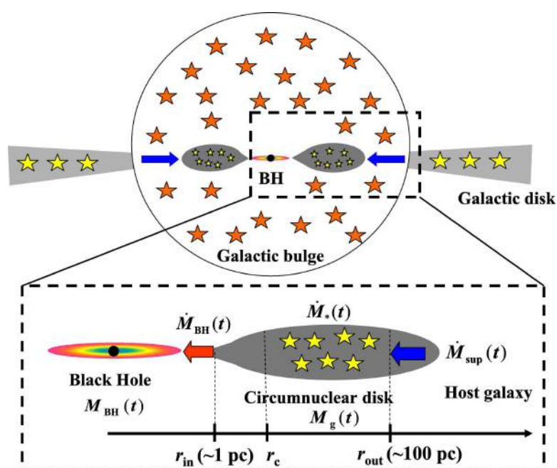
Figure 6.1: SMBH growth schematic diagram - The figure represents the model of a circumnuclear disk supported by the turbulent pressure via supernova explosions. M_{\text{BH}} , M_{\text{g}} , \dot{M}_{\text{BH}} , \dot{M}_{*} and \dot{M}_{\text{sup}} are the mass of the SMBH, the gas mass, the stellar mass, the BH growth rate, the star formation rate, and the mass supply rate from the host galaxy, respectively. From Kawakatu & Wada (2008).
