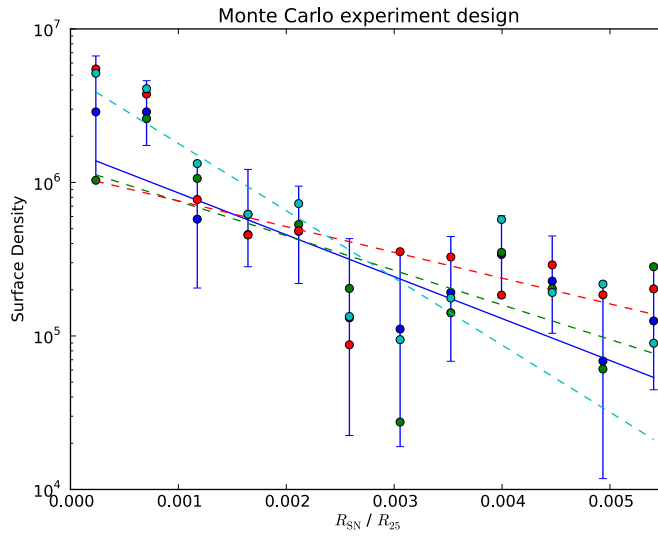
Figure 6.3: Illustration of the designed Monte Carlo experiment - Original points, error bars and fit are plotted in blue. New sets of points (in other colors) were chosen randomly within the error bar of each original point and fits were made for each data set (dashed lines). If the fitting algorithm did not converge or if its standard deviation was over 5 times the fitting value, the set was discarded and a new one was generated. Only three extra fits are shown here for the sake of clarity, but a total of 10 000 data sets were generated for each nuclear starburst studied.
