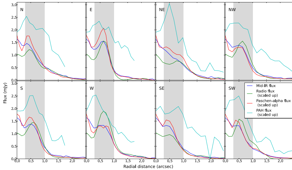
Figure 3.2: Azimuthal profile of the fluxes - Mid-IR ( 8.7 \mu\text{m} , in blue), radio (3.6 cm from Nov 2004, in green), \text{Pa}\alpha ( 1.9 \mu\text{m} , in red) and continuum-subtracted PAH feature ( 3.3 \mu\text{m} , in cyan), starting from the center of the images. Radio, \text{Pa}\alpha and PAH fluxes are scaled up by the median of the 8.7 \mu\text{m}/3.6 \text{ cm} , 8.7 \mu\text{m}/\text{Pa}\alpha and 8.7 \mu\text{m}/3.3 \mu\text{m} ratios, respectively (factors 19.2, 10.8 and 13.6). The profile is shown for eight cardinal directions, with an azimuthal binning of the size of a pixel ( 0.116'' for the 3.3 \mu\text{m} image and 0.089'' for the other cases). The shaded area, from 0.3 to 1.0 arcsec, corresponds to the approximate width of the star formation ring.
