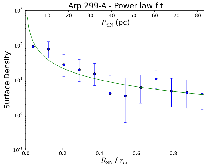
Figure 6.7: Arp 299-A power law fitting - Surface density of SNe vs radius, normalized to the furthest source, r_{\text{out}} , in Arp 299-A and non-linear fit to a power law with \gamma = 1.1 .
