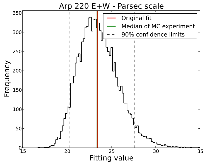
Figure 6.13: Monte Carlo results for combined nuclei in Arp 220 - MC histogram for the fitting of the combined SN sample of both East and West nuclei in Arp 220. The resulting scale length is h_{\text{SN}} = 23.4 pc.
