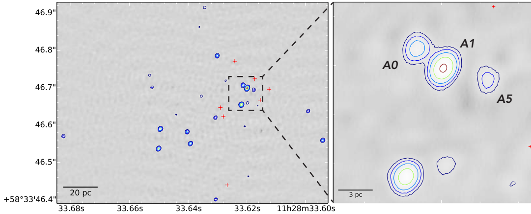
Figure 5.6: Arp 299-A EVN image stacking at 5 GHz - Beam size is 10 \times 8 \text{ mas} , \text{PA} = -25^\circ . The noise of the image is 18.5 \mu\text{Jy beam}^{-1} and contours are plotted at (5, 9, 15, 27, 45) \times \text{rms} . Red crosses indicate the position of the additional compact sources found by Ulvestad (2009) at 2.3 and 8.4 GHz. Right panel is a zoom to the image, showing the low-luminosity AGN (A1) and its jet (A5), and the closest supernova to the AGN (A0).
