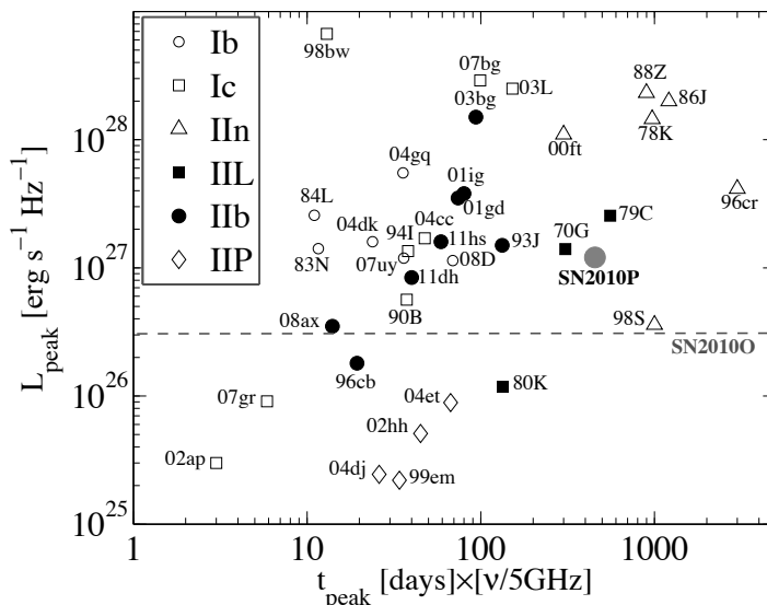
Figure 5.5: Peak monochromatic luminosity vs time to peak from explosion date - SN from different types are plotted together with SN2010P. The dashed line shows the upper luminosity limit for SN2010O. From Romero-Cañizales et al. (2014).
