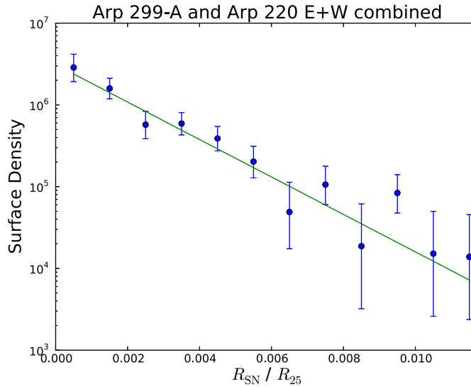
Figure 6.16: Surface density combined profile of Arp 299-A and Arp 220 - Non-linear fit for the combined sources from both Arp 299-A and Arp 220. The scale length is \tilde{h}_{\text{SN}} = 2.0 \times 10^{-3} .
